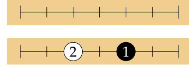
Figure 3.9 – Empty board and board with a black and a white stone.
