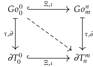
Figure 3.12 – Diagram of the complete structure. The horizontal arrows ( \Xi ) expand dimensions and players ( l ). The vertical ones ( \tau ) close the space, and ( \partial ) hollow out the interior.
